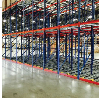
Heavy Duty Pallet Rack System
