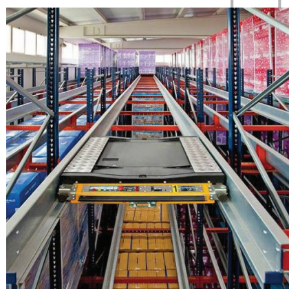
Pallet Racking Radio Shuttle Shelf
