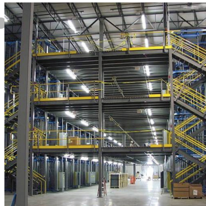
Rack Support Mezzanine Floor for Warehouse
